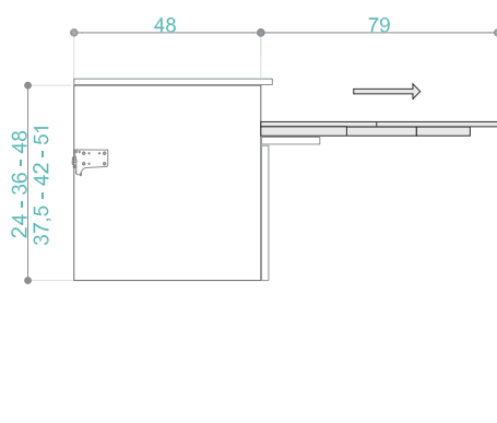
VISTA LATERALE SIDE VIEW
