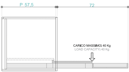
VISTA LATERALE SIDE VIEW
